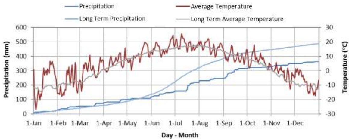
Figure 15. Actual precipitation and temperature data for 2015 compared to normals at Stony Plain. (data from Alberta Agriculture, 2015)
