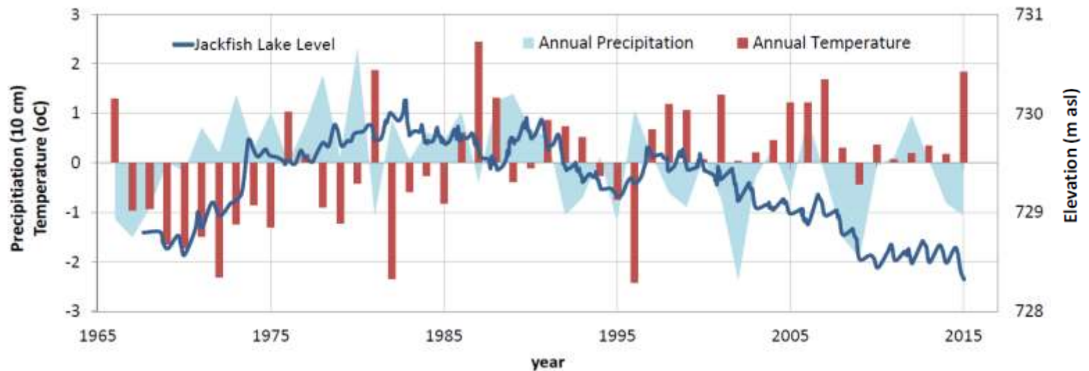
Figure 48. Jackfish Lake water levels compared to annual precipitation and temperature at Stony Plain (data from Alberta Environment and Parks, 2015b and Environment Canada, 2015)
