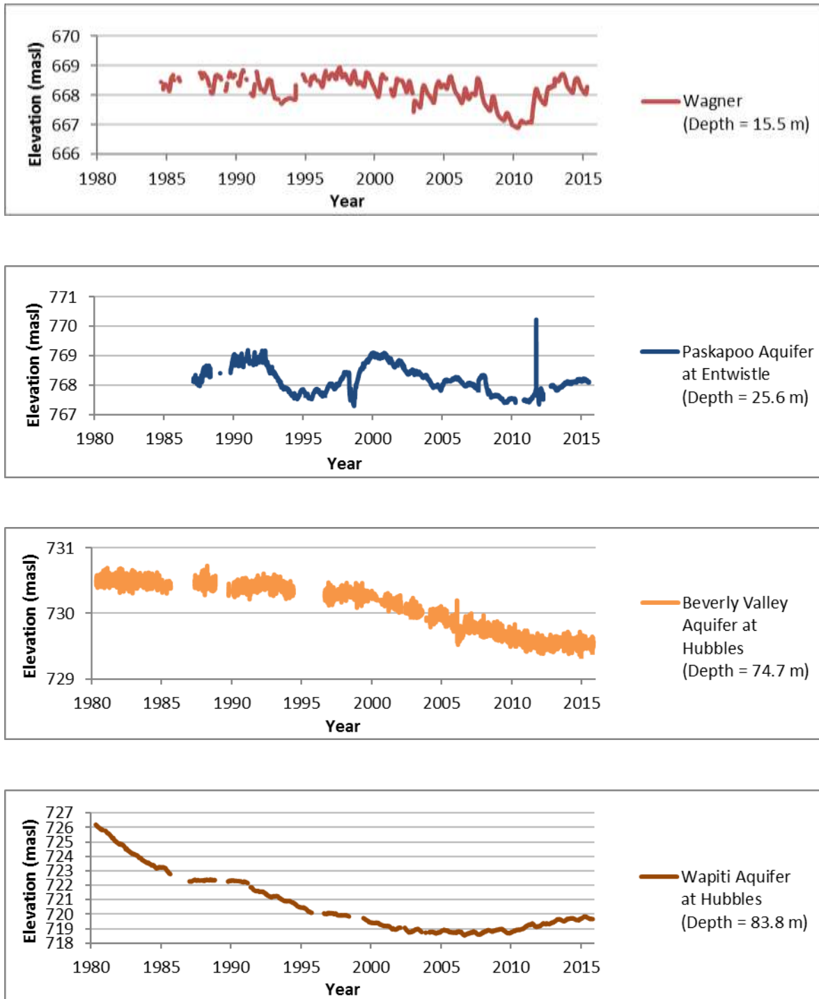
Figure 28a. Groundwater levels from 1980 to 2015 at Wagner Natural Area, Entwistle and Hubbles Lake (data from Alberta Environment and Parks Groundwater Observation Well Network, 2015b).
