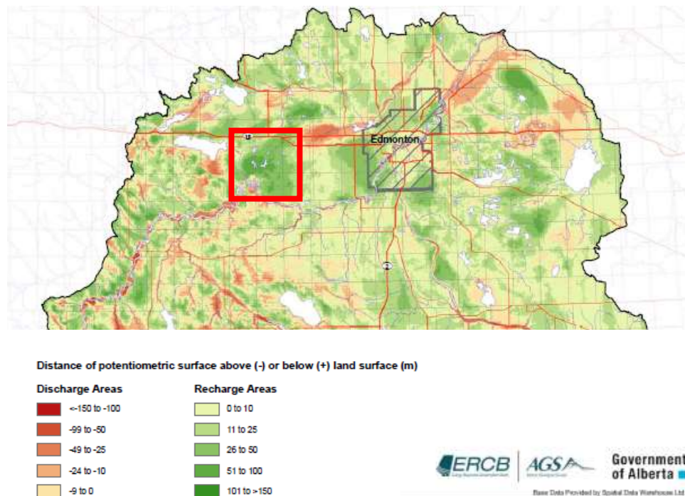
Figure 25. Recharge and discharge potentials in the Edmonton area. The approximate location of Jackfish Lake is indicated by the red square (Barker et al., 2011)
