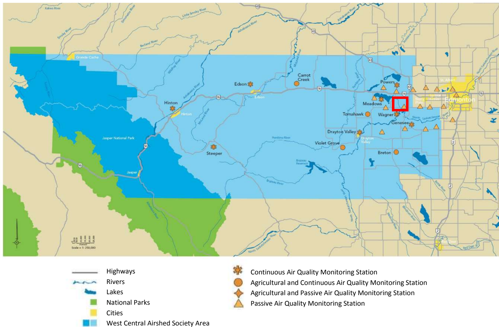
Figure 43. West Central Airshed Society boundaries and stations. The red square indicates the approximate location of Jackfish Lake. (adapted from West Central Airshed Society, 2013)
