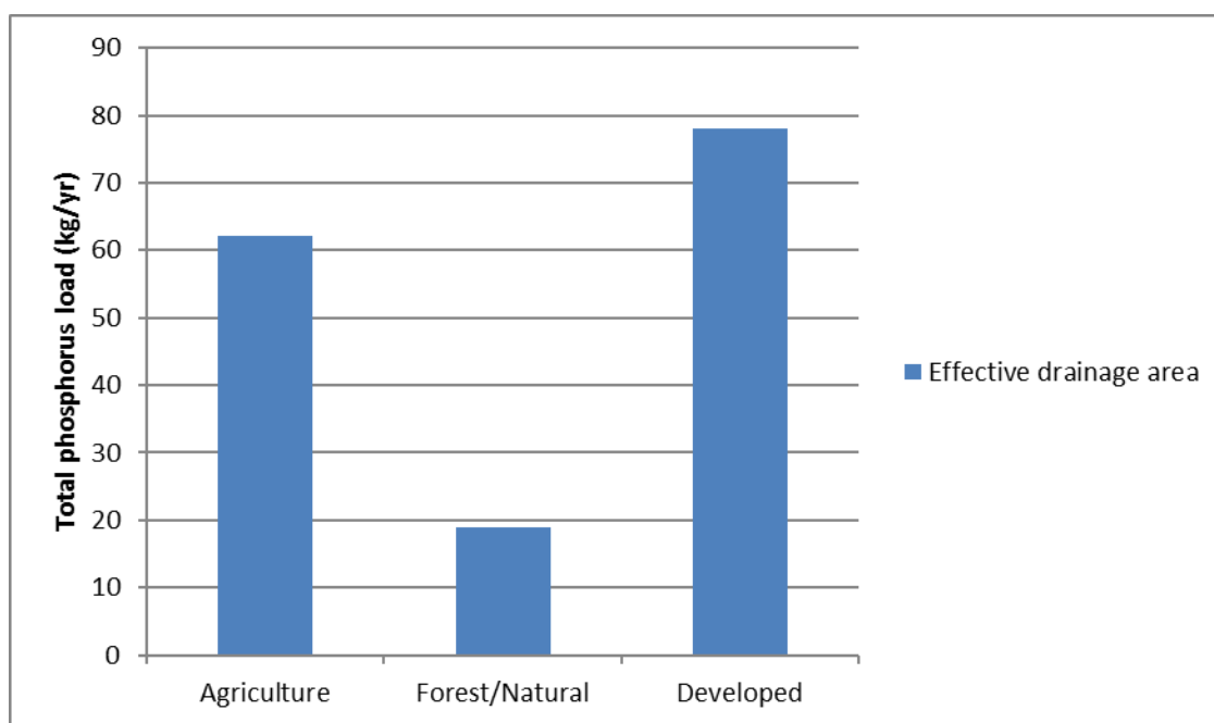
Figure 6: Total Phosphorus loads from the effective drainage area of Jackfish Lake (EDA)
