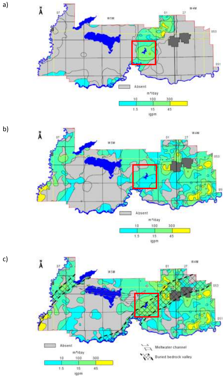
Figure 29. Apparent yield for (a) upper (b) lower and (c) all water wells completed through sand and gravel aquifers in Parkland County. The approximate location of Jackfish Lake is indicated by the red squares (Hydrogeologic Consultants Ltd., 1999).
