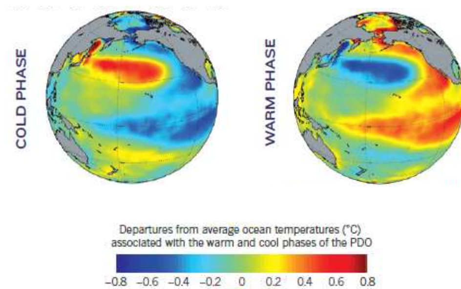
Figure 19. Phases of the Pacific Decadal Oscillation (Tollefson, 2014)
