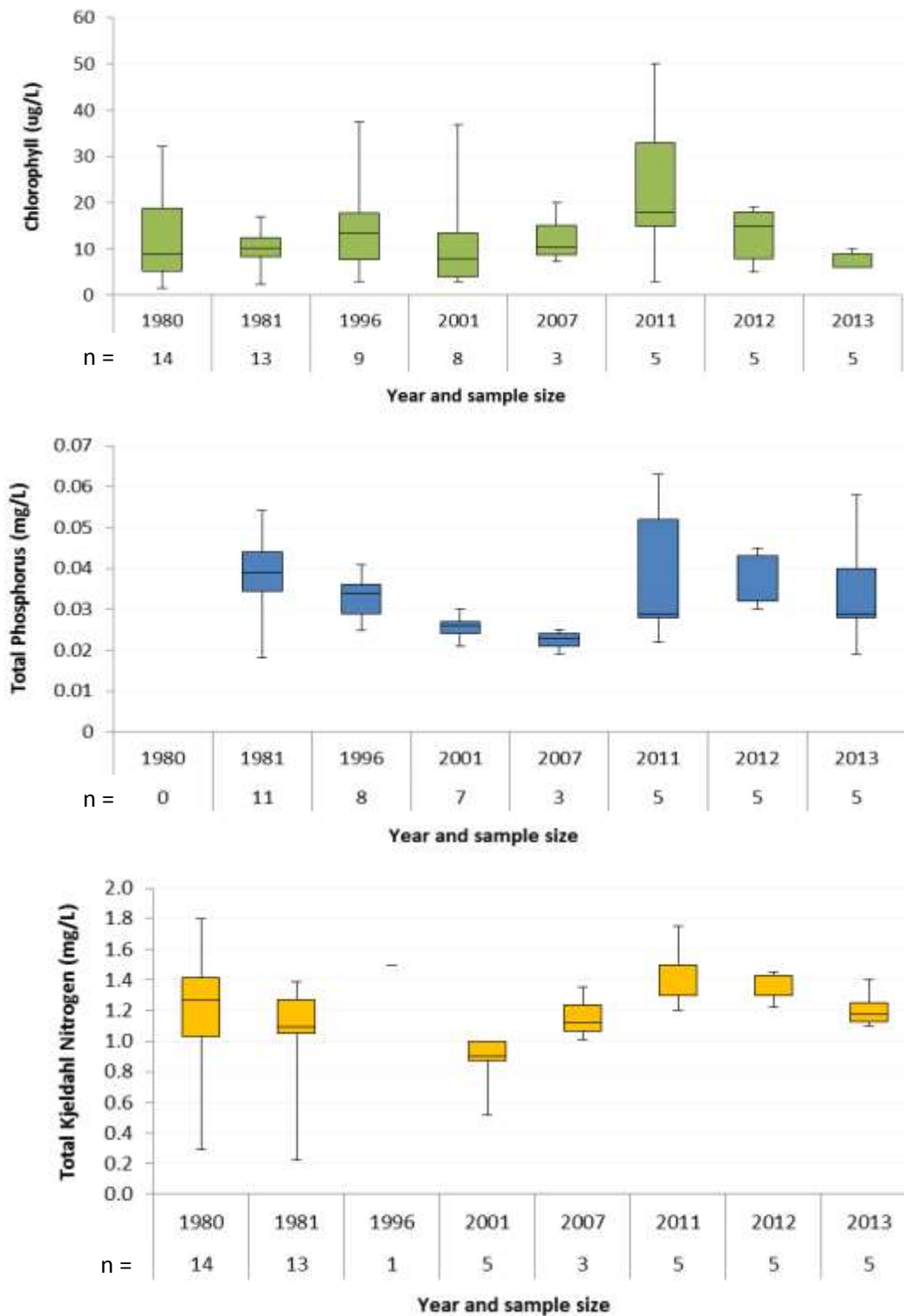
Figure 52. Annual ranges for chlorophyll-a, total phosphorus and total kjeldahl nitrogen in Jackfish Lake during the open water season (Alberta Environment and ALMS, 1980-2013)
