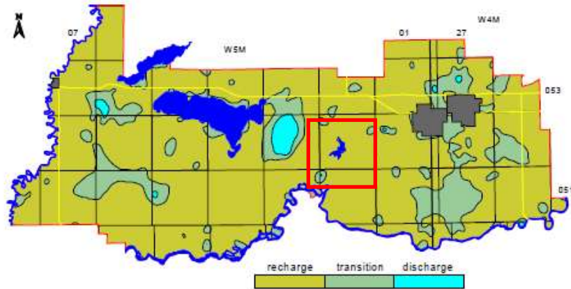
Figure 24. Groundwater recharge, discharge and transition areas in Parkland County. The approximate location of Jackfish Lake is indicated by the red square (Hydrogeologic Consultants Ltd., 1999).
